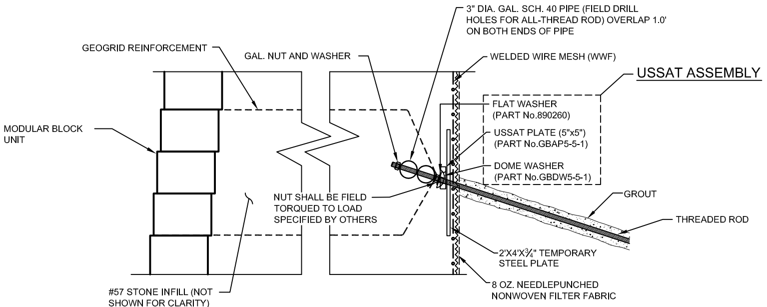
ANCHOR HEAD CONNECTION DETAIL THREADED ROD NOT TO SCALE
